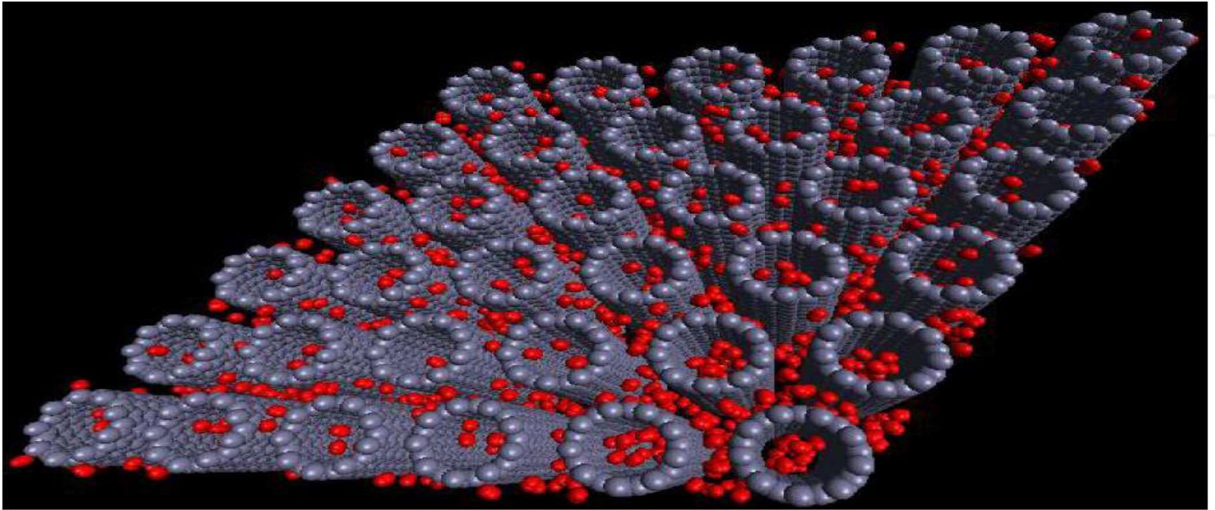
Figure 7. Hydrogen gas (red) adsorbed in an array of carbon nanotubes (grey). The hydrogen inside the nanotubes and in the interstitial channels is at a much higher density than that of the bulk gas.
