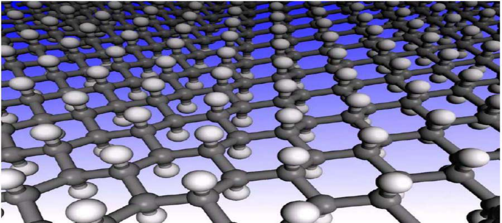
Figure 8. Structure of graphane in the chair conformation. The carbon atoms are shown in gray and the hydrogen atoms in white.
