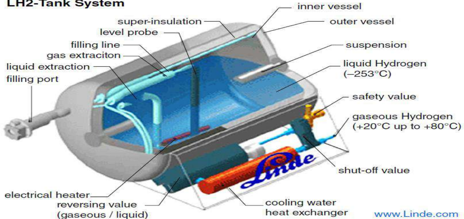
FIGURE 5. Schematic illustration of a representative cryogenic vessel (Liquid hydrogen storage tank system, horizontal mounted with double gasket and dual seal )
